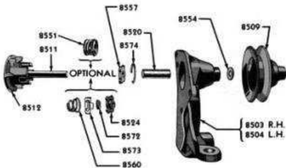
1937-48 8 CYL. 90 & 100 H.P. PASSENGER, COMMERCIAL & TRUCK WATER PUMP (78-8501-2)
